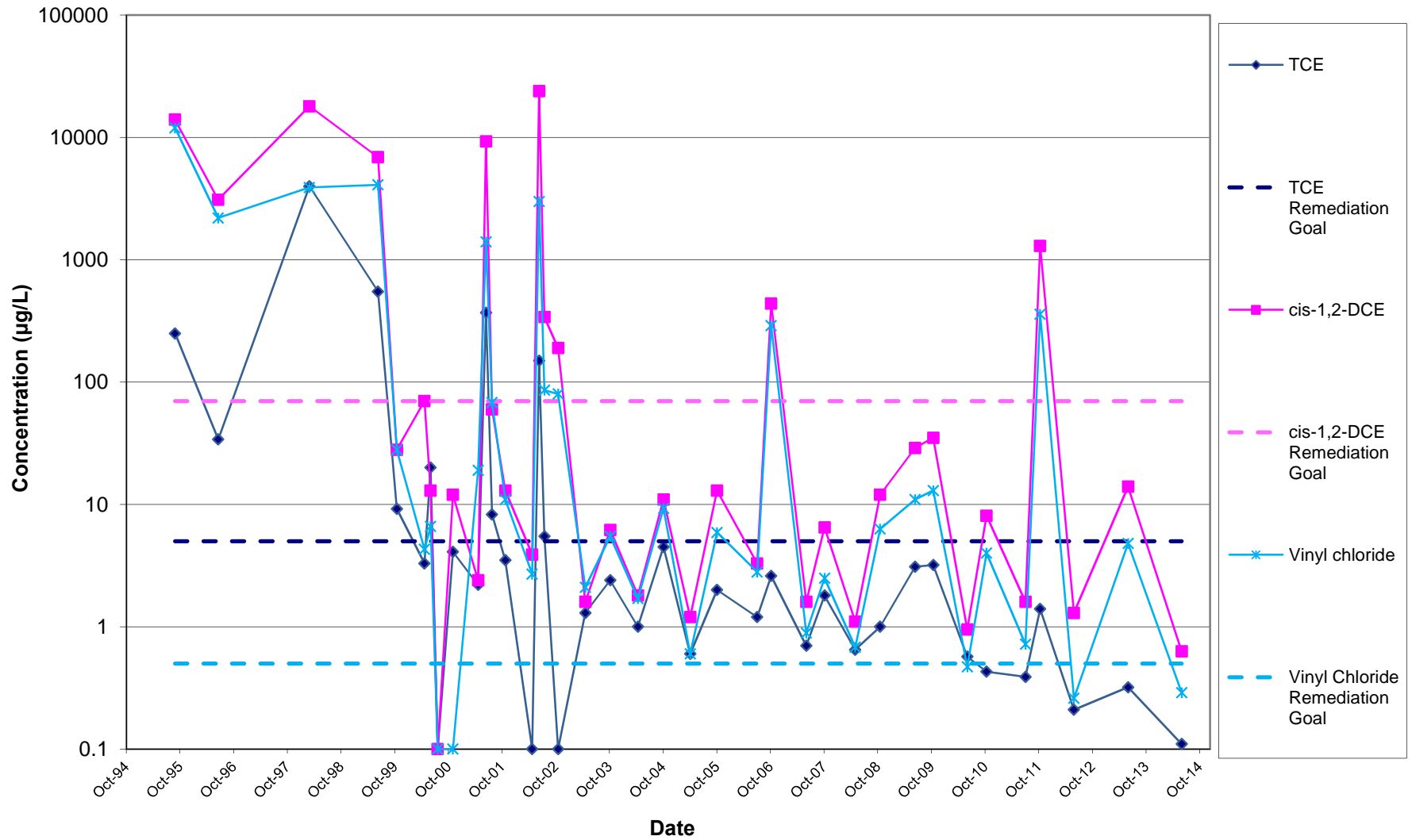
Figure D-5a. South Plantation MW1-16 VOC Trends
