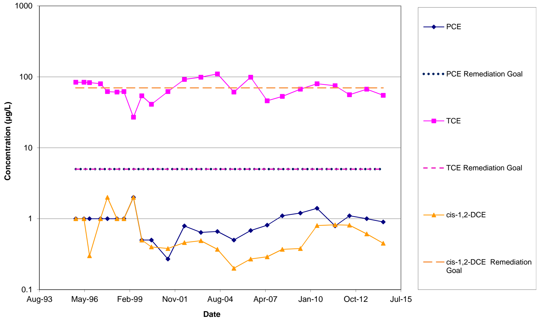
Figure D-19a. Area 8 MW8-11 VOC Trends
