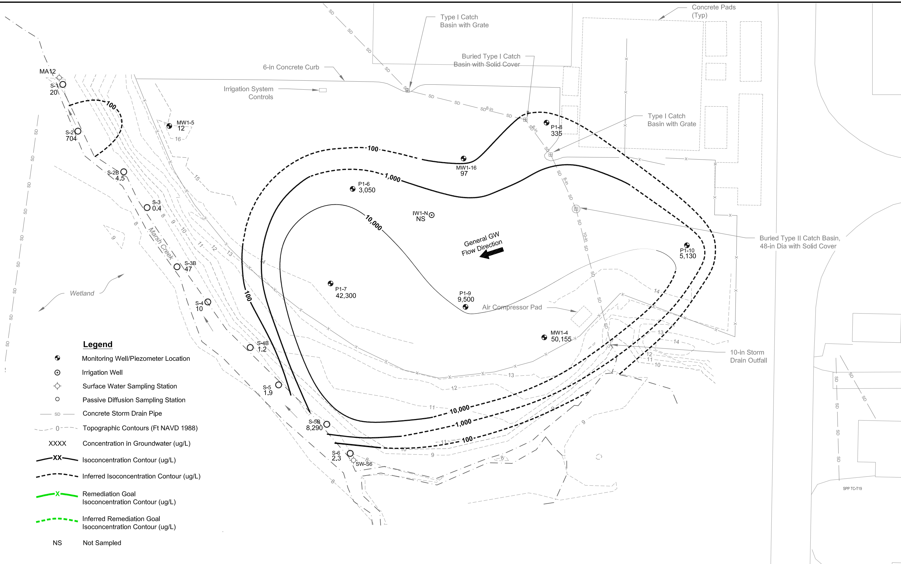
Figure C-35 OU 1, CVOCs Groundwater Concentrations, South Plantation Upper Aquifer, 2010
