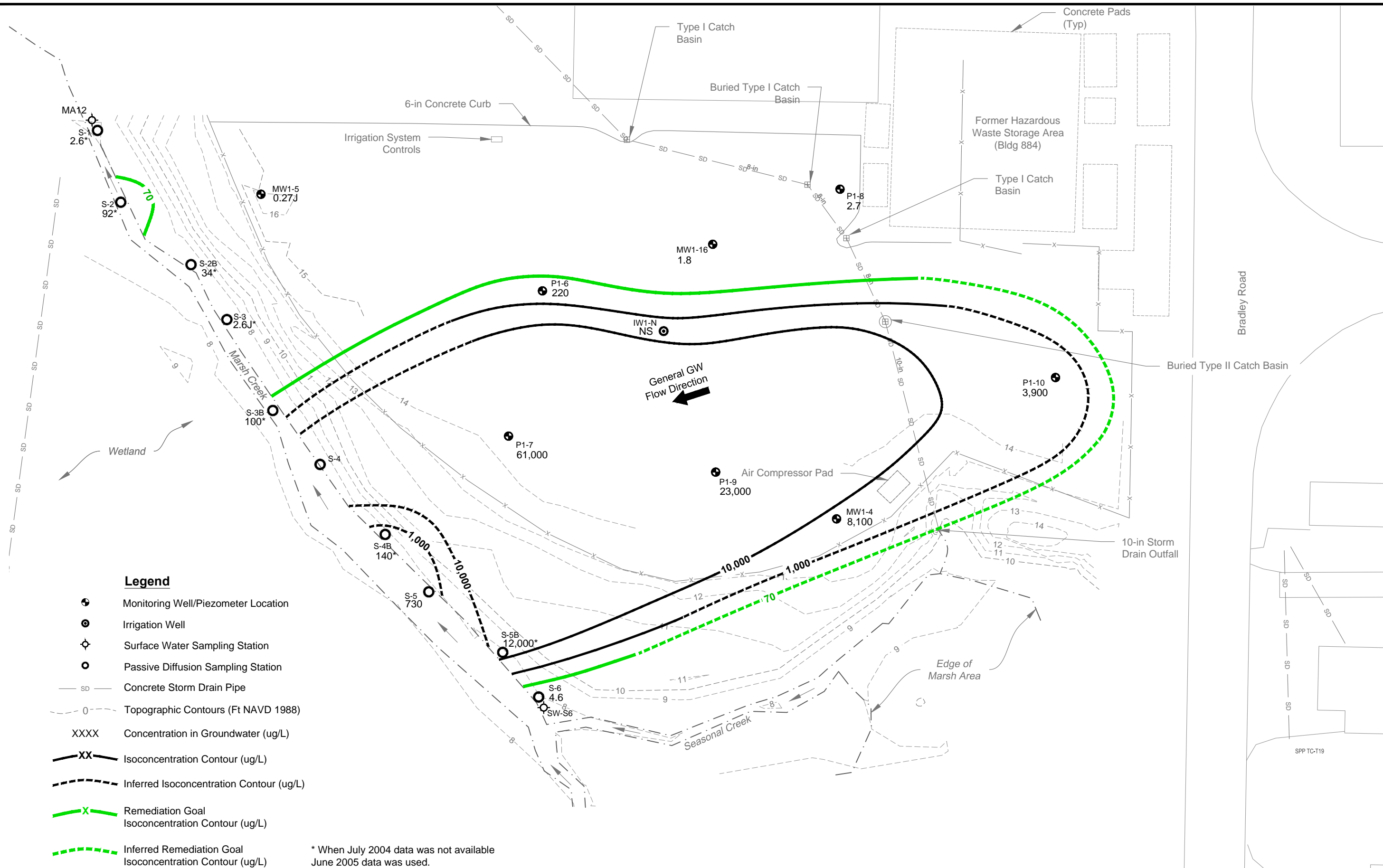
Figure C-26 OU 1, cis-1,2-DCE Groundwater Concentrations, South Plantation Upper Aquifer, 2004/2005
