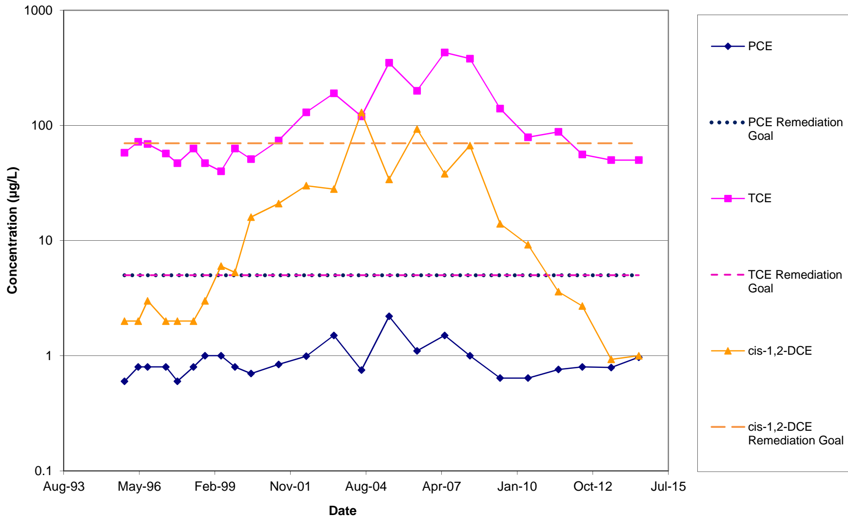
Figure D-21a. Area 8 MW8-16 VOC Trends
