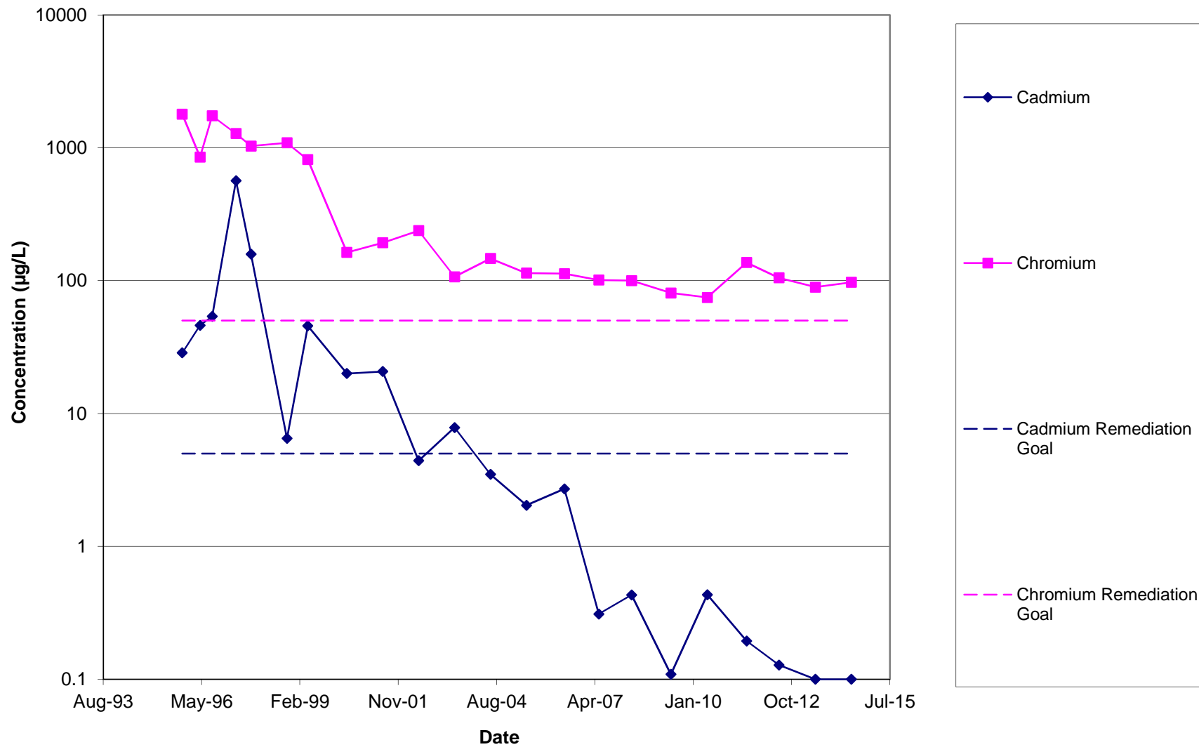
Figure D-20b. Area 8 MW8-12 Cd and Cr Concentration Trends
