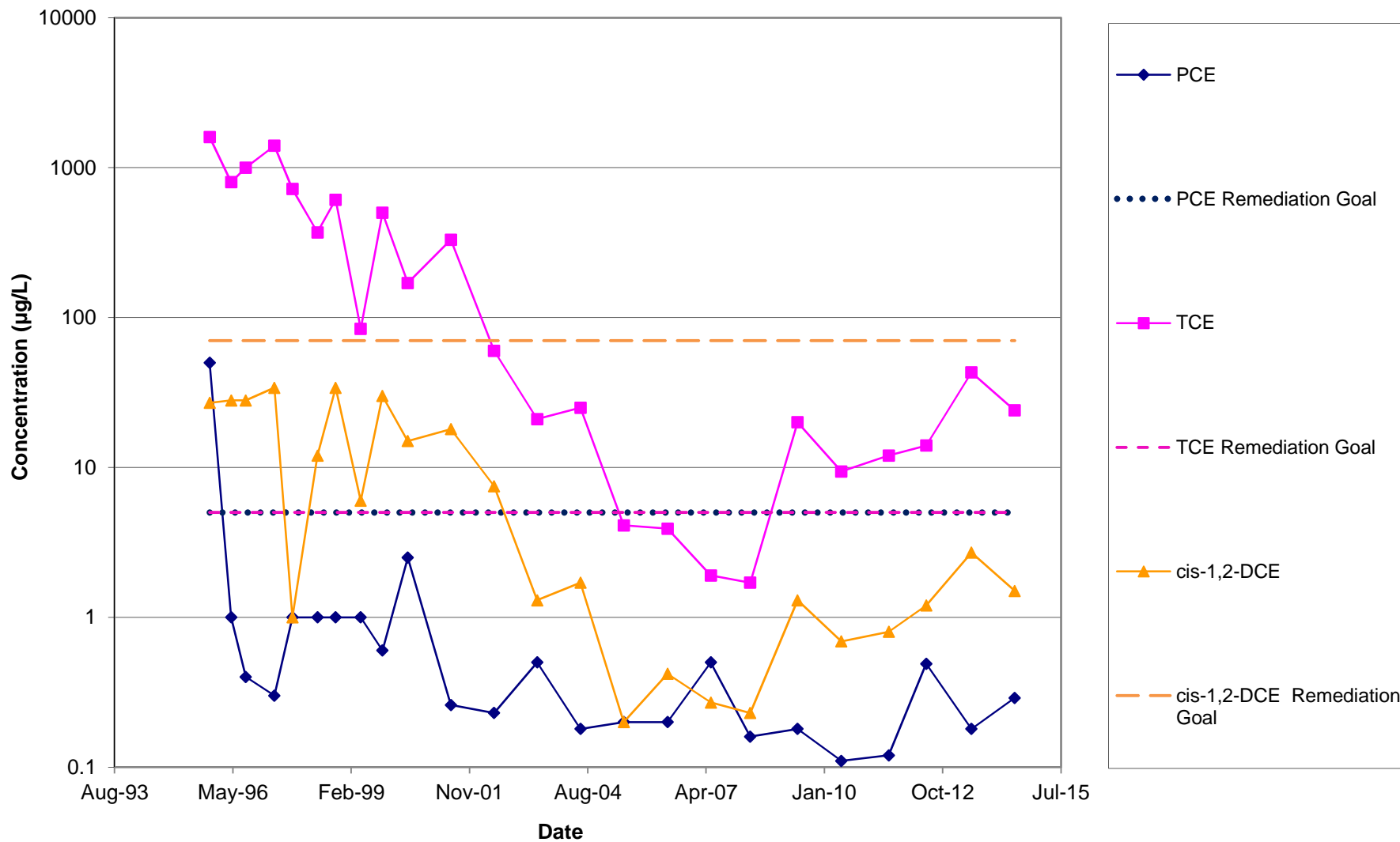
Figure D-18a. Area 8 MW8-9 VOC Trends
