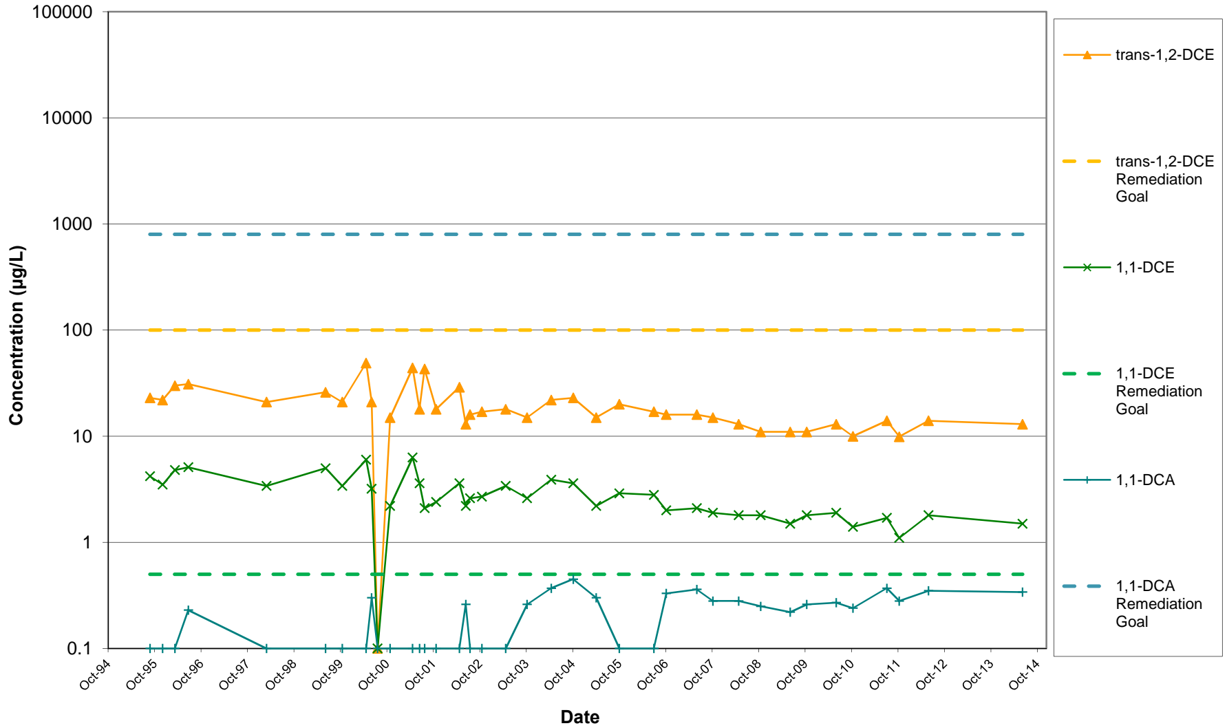
Figure D-2b. North Plantation MW1-2 VOC Trends
