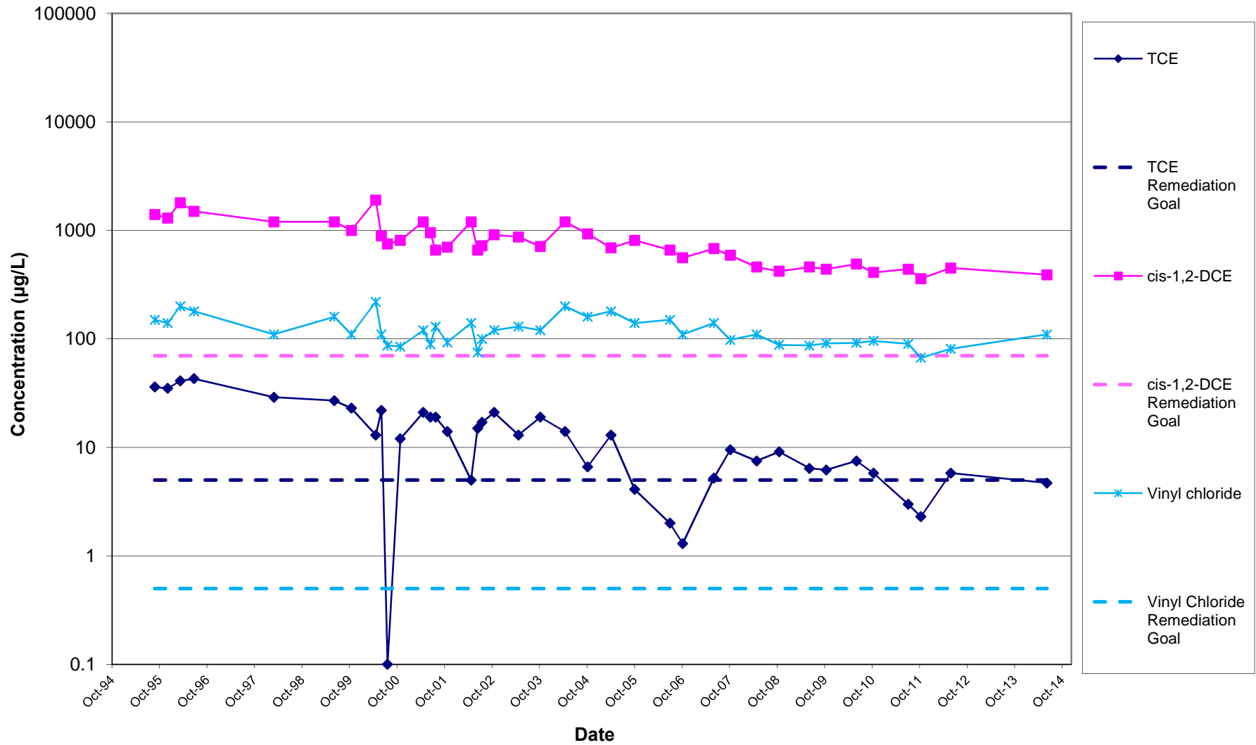
Figure D-2a. North Plantation MW1-2 VOC Trends
