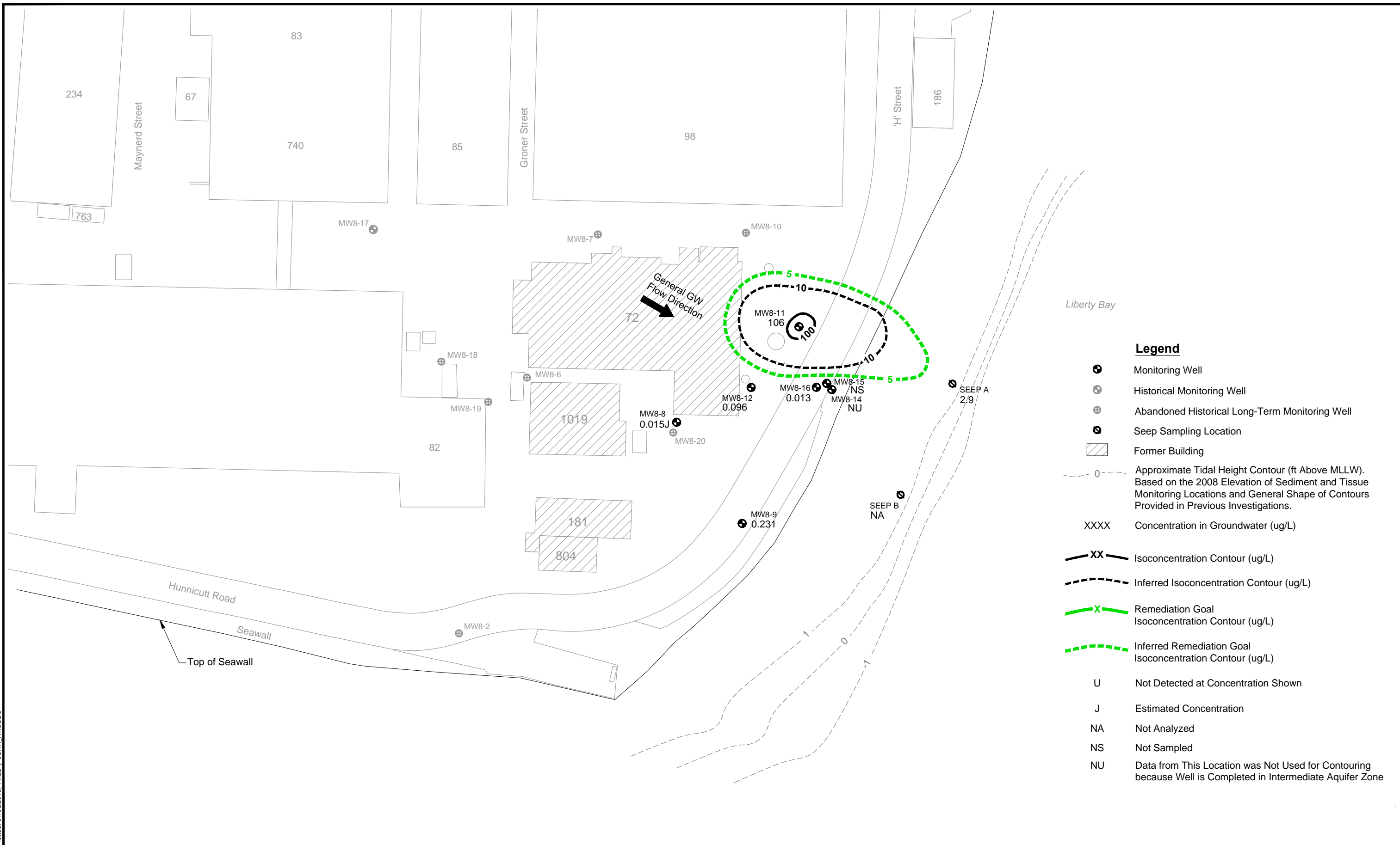
Figure C-60 OU 2, Area 8 Dissolved Cadmium Groundwater Concentrations, June 2014
