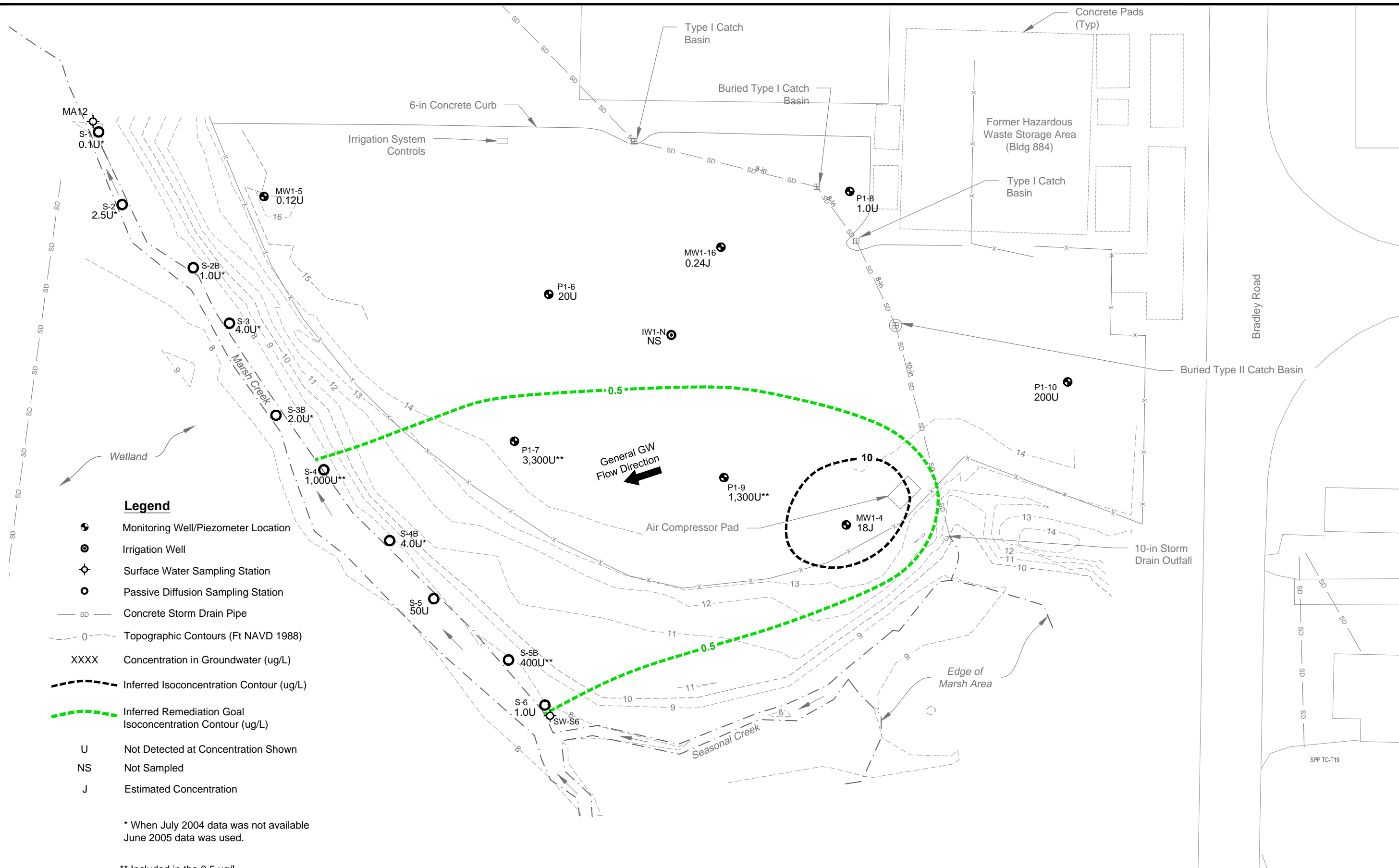
Figure C-22 OU 1, 1,1-DCE Groundwater Concentrations, South Plantation Upper Aquifer, 2004/2005
