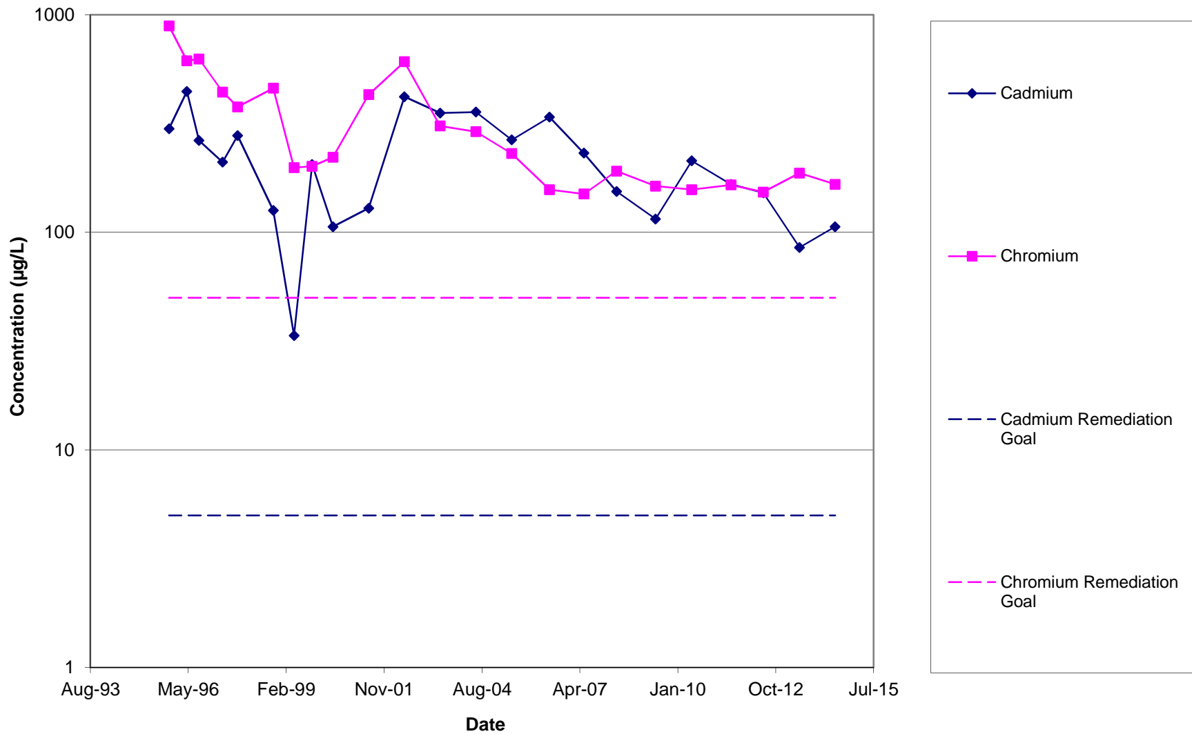
Figure D-19b. Area 8 MW8-11 Cd and Cr Concentration Trends
