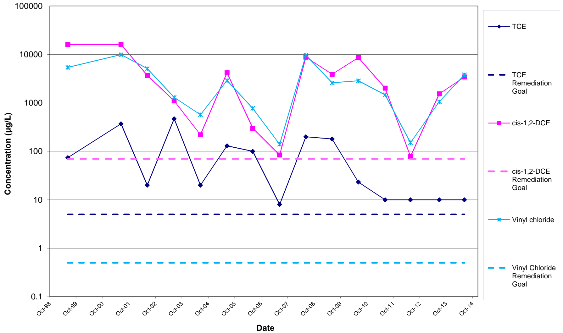
Figure D-6a. Area 1 South Plantation P1-6 VOC Trends
