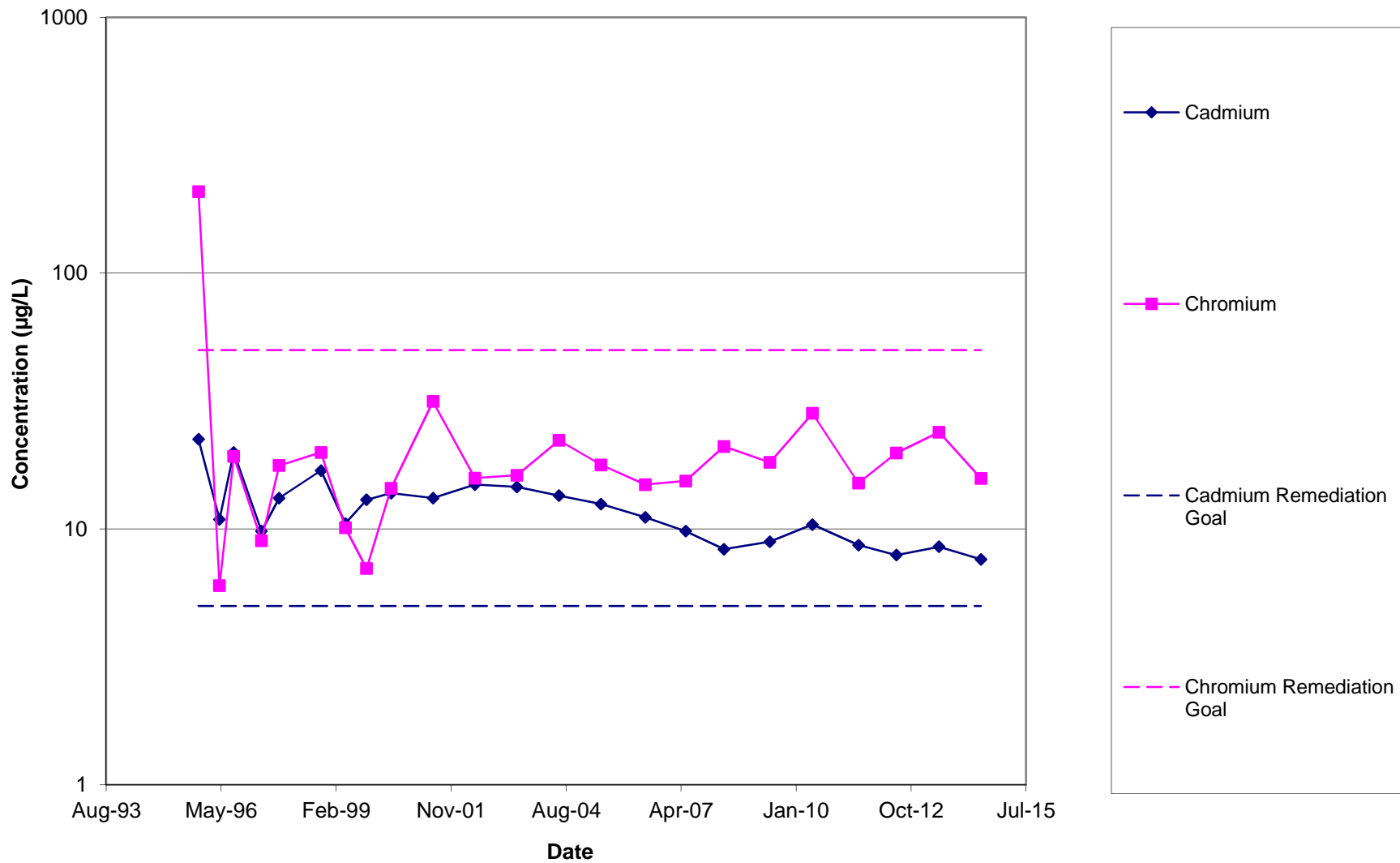
Figure D-21b. Area 8 MW8-14 Cd and Cr Concentration Trends
