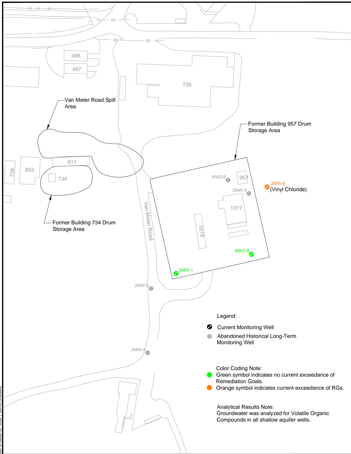
Figure 6-3 2014 Monitoring Locations at OU 2 Area 2
