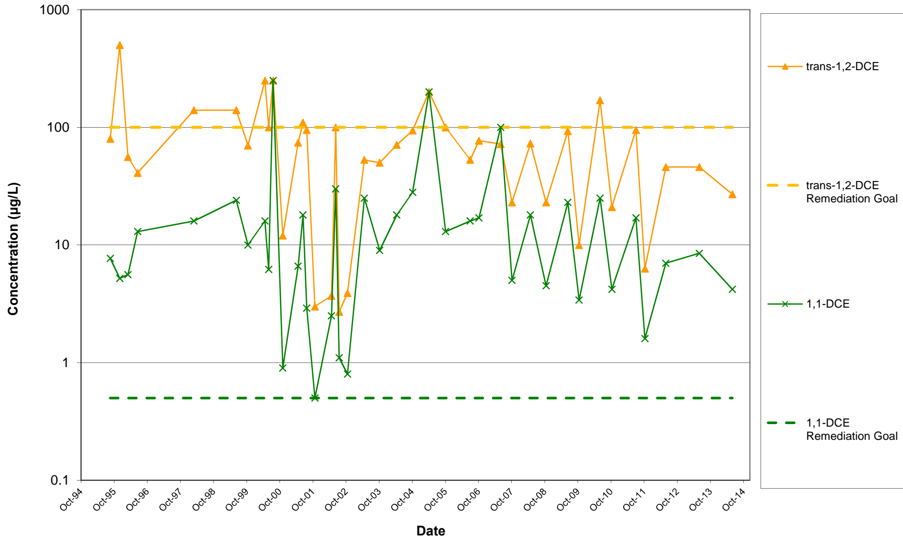
Figure D-3b. South Plantation MW1-04 VOC Trends
