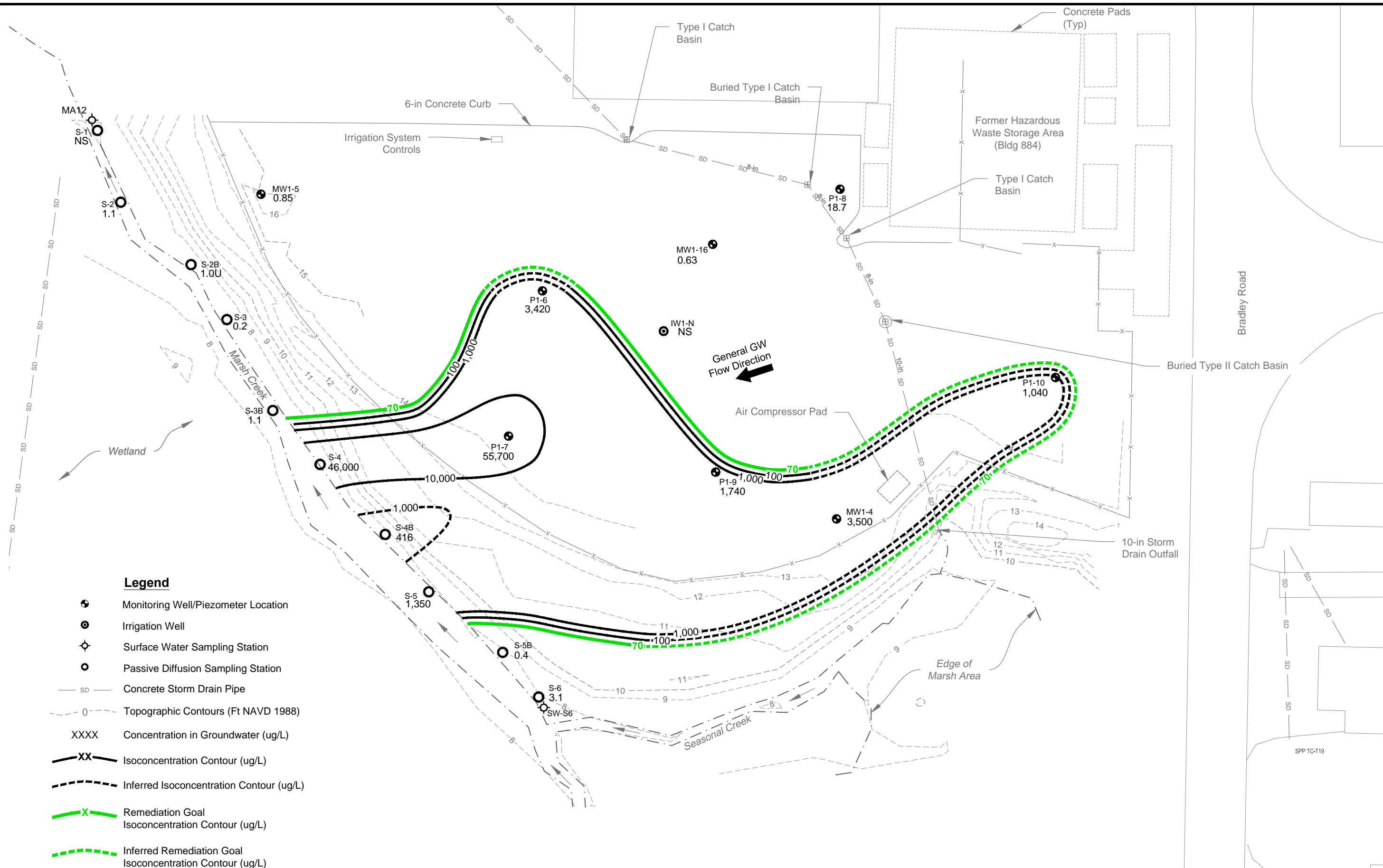
Figure C-28 OU 1, cis-1,2-DCE Groundwater Concentrations, South Plantation Upper Aquifer, 2014
